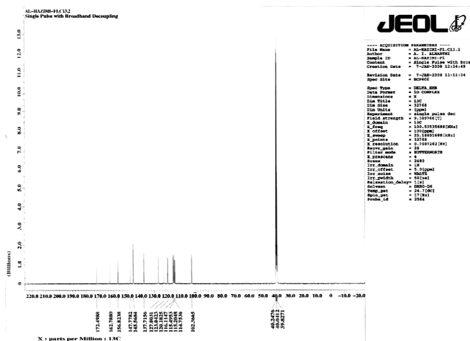
Figure 2 The ^{13}\text{C} -NMR chemical shift of flavonoid compound 1 in \text{DMSO-d}_6 .
